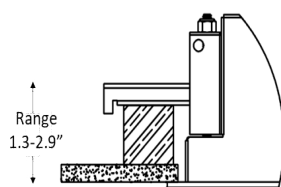
Inset Door Flanged (Framing by others)
